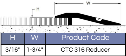
316 REDUCER WITH OR WITHOUT HOLES
