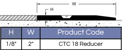
18 REDUCER WITH OR WITHOUT HOLES
